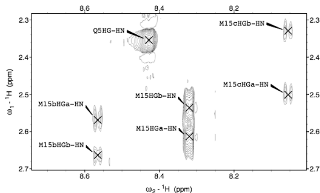
FIGURE 3: The H^\beta – H^N connectivity region of a ^1\text{H} – ^1\text{H} total correlation spectroscopy (TOCSY; 60 ms mixing time, DIPSI spin-lock, 800 MHz field strength) experiment acquired for apelin-17 ( \sim 3.5 mM peptide in 20 mM \text{Na}^+\text{CD}_3\text{COO}^- buffer at pH 5.00 \pm 0.05 prepared in 90% \text{H}_2\text{O}/10\% \text{D}_2\text{O} with 1 mM \text{NaN}_3 and 1 mM DSS) at 35 °C.
