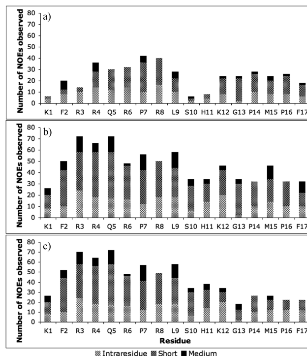
FIGURE 4: A breakdown of nuclear Overhauser effect (NOE) contacts per amino acid residue used to calculate the final ensembles of structures, with short (sequential) and medium ( |i - j| \leq 4 ) NOE interactions shown for apelin-17 at 35 °C (a) and for conformers A and B at 5 °C (shown in (b) and (c), respectively). Note that these plots do not include ambiguous NOEs shown in Table 2.
