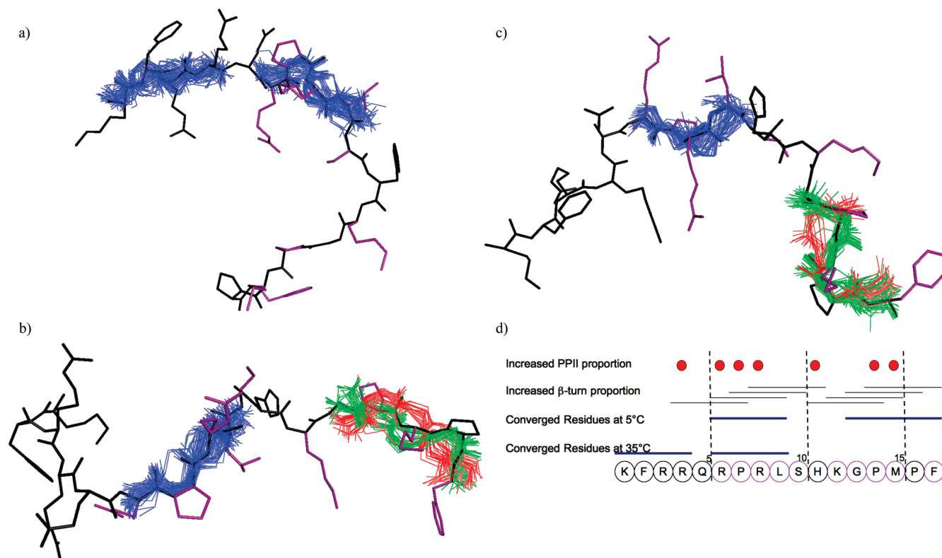
FIGURE 7: Representative structures for apelin-17 structural ensembles (a) at 35 °C, (b) of the primary conformer (conformer A; trans peptide bonds at P14 and P16) at 5 °C and (c) of the second most populated conformer (conformer B; cis peptide bonds at P14 and P16) at 5 °C are shown in stick form for backbone and side chains. A summary of structural properties is provided in (d) relative to the apelin-17 sequence. For structurally converged regions (identified for each temperature in (d)), the backbones of all 80 ensemble members are shown superposed over the representative structure. Ensemble members are colored by cluster for the C-terminus of (b and c), where major clusters of backbone conformation exist. Functionally critical residues (11–13, 49, 50) identified by Ala-substitution studies are colored purple, both for side chains in (a–c) and for the circle surrounding the residue in (d). Increased polypyrrolidine-II (PP II ) and \beta -turn abundance based on parallel examination of all three ensembles (detailed in Figure 6) are indicated, with all four residues involved in a given \beta -turn indicated by a bar covering those residues.
